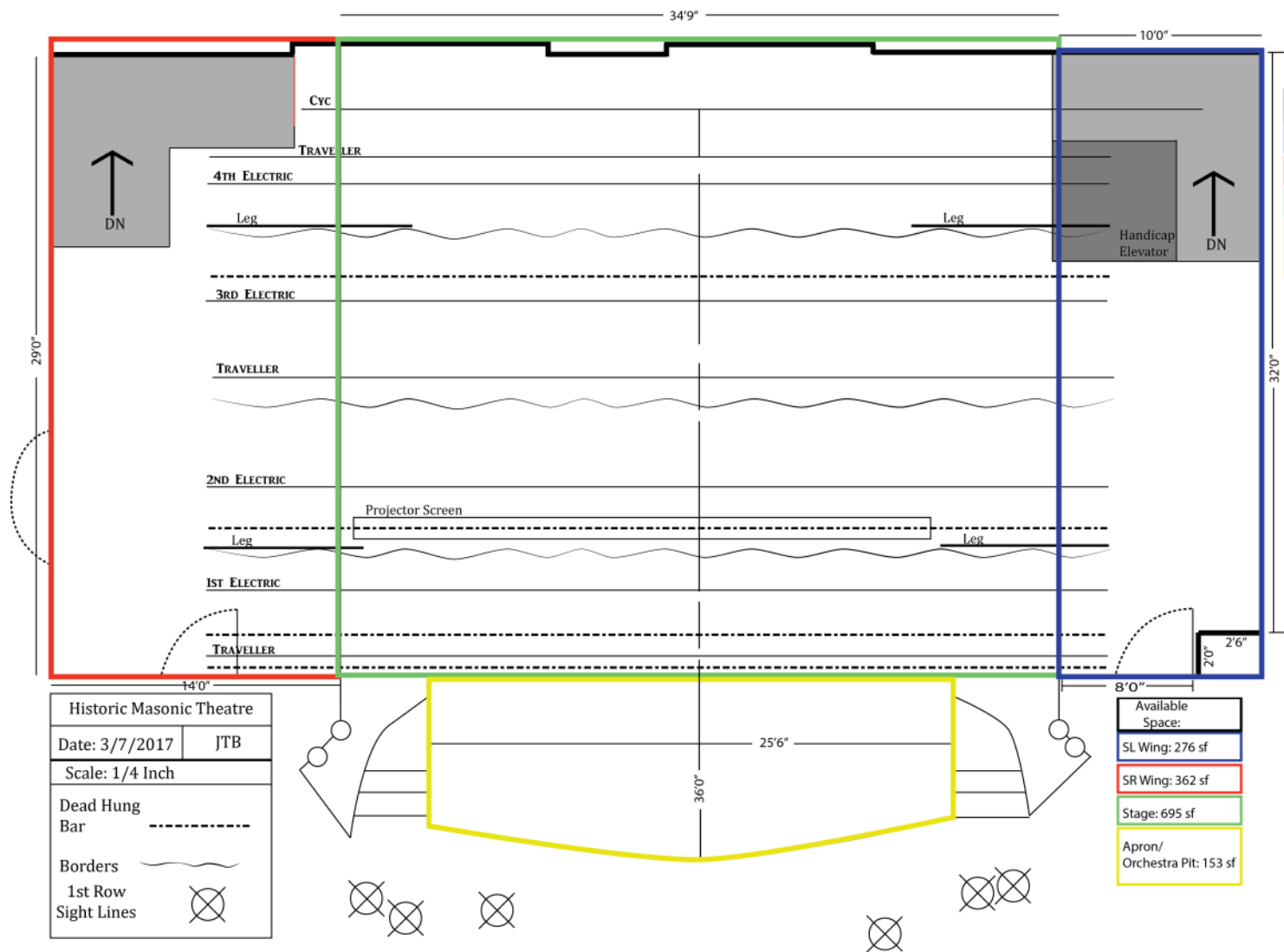
Auditorium Stage Groundplan
